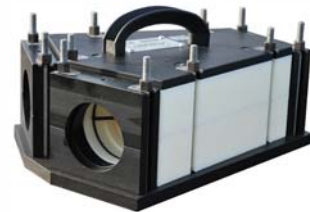
Y-connector, for the installation of cable into an occupied duct
